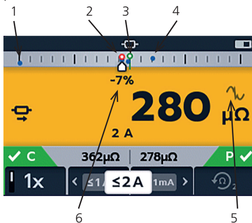
DLRO2 colour display with new Difference Meter
