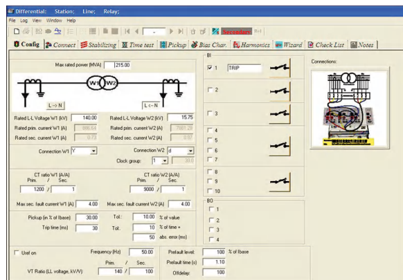
Differential instrument
